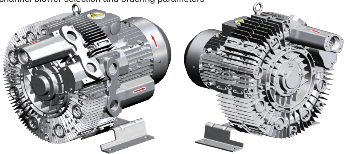
气环风机的选型和订购参数 Side channel blower selection and ordering parameters
